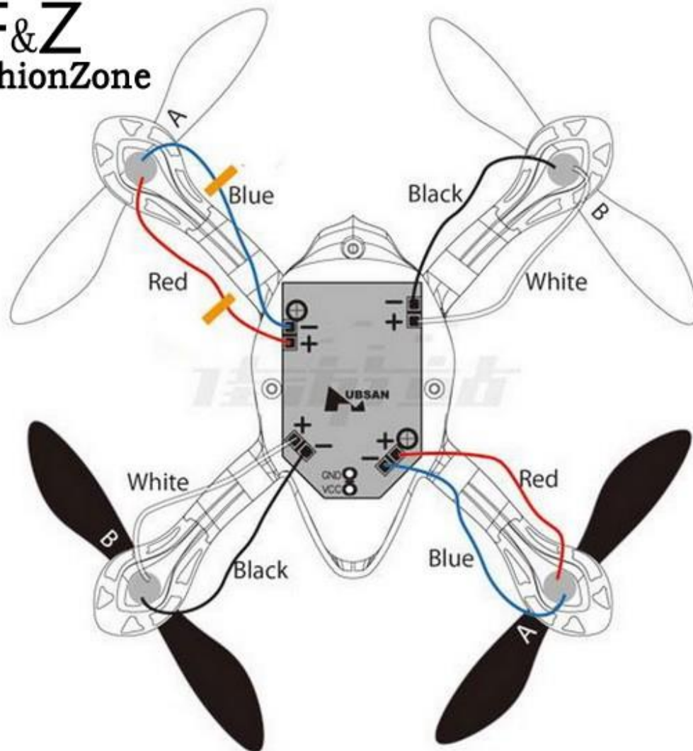
(Bottom View)
